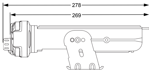
Figure 1-10. Side View of O2 Control Head Attached to APX 7500 Mid Power Dash Mount Transceiver and Trunnion
