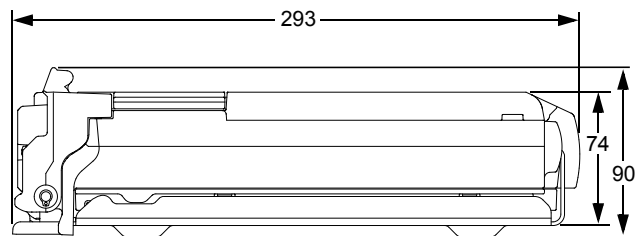
Figure 1-8. Side View of APX 7500 High Power (100W) Transceiver and Trunnion
