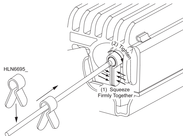
Figure 2-53. Mini-UHF Connector Tool (100W Radios Only)
