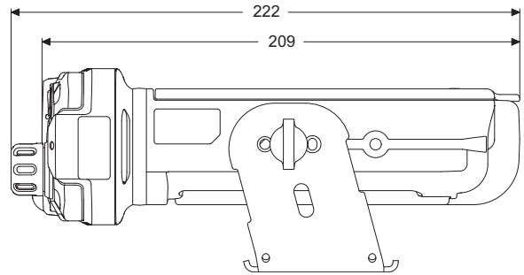
Figure 1-6. Side View of APX 2500/APX 4500/APX 1500 Mid Power Dash Mount Transceiver and Trunnion
