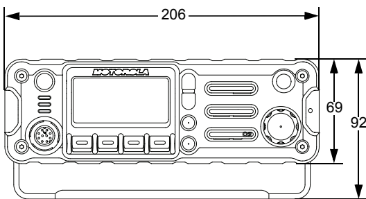
Figure 1-9. Front View of O2 Control Head Attached to APX 7500 Mid Power Dash Mount Transceiver and Trunnion
