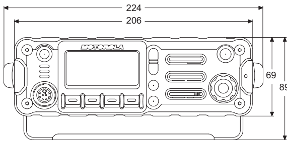
Figure 1-5. Front View of APX 2500/APX 4500/APX 1500 Mid Power Dash Mount Transceiver and Trunnion
